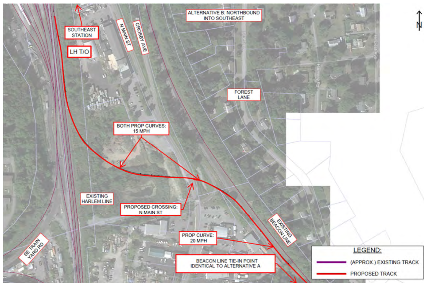
FIGURE 29. BEACON-HARLEM LINE CONNECTOR - ALTERNATIVE B
