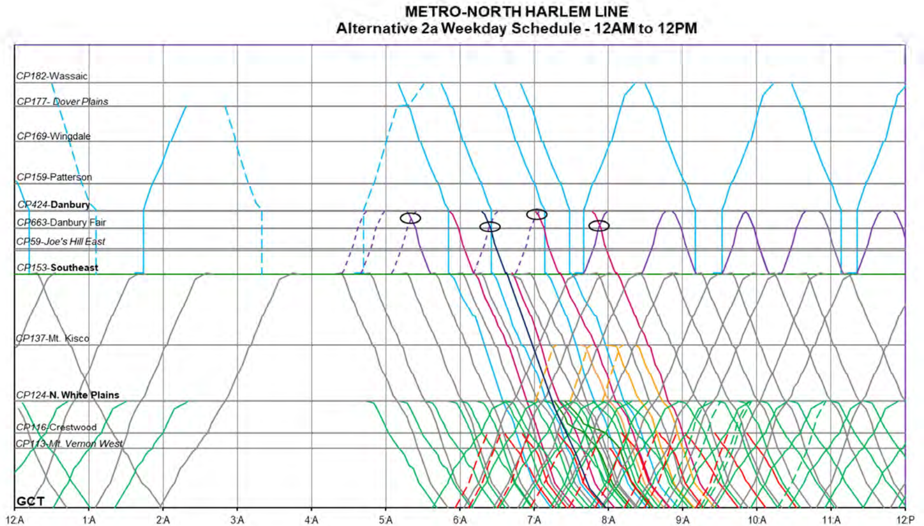
FIGURE 53. ALTERNATIVE 2 STRINGLINE DIAGRAM – 12AM TO 12 PM
