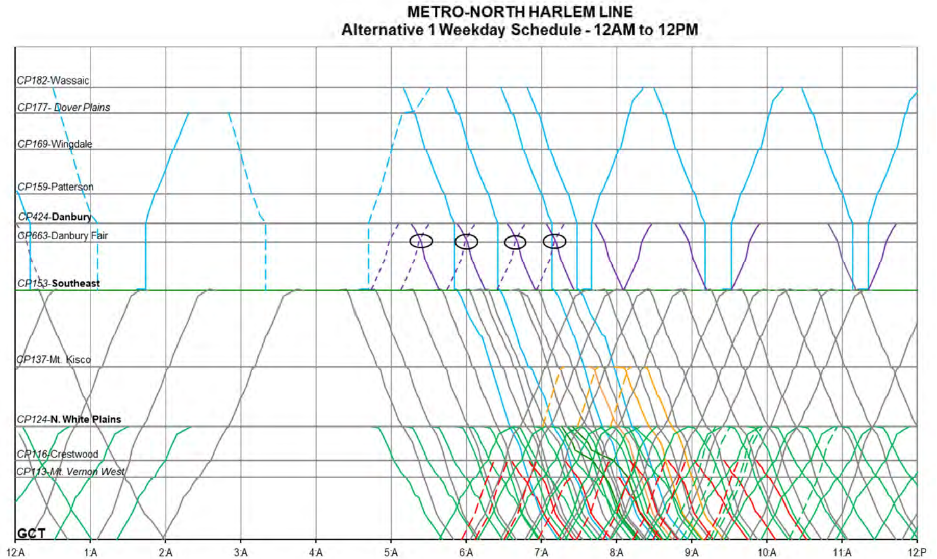
FIGURE 51. ALTERNATIVE 1 STRINGLINE DIAGRAM – 12AM TO 12 PM
