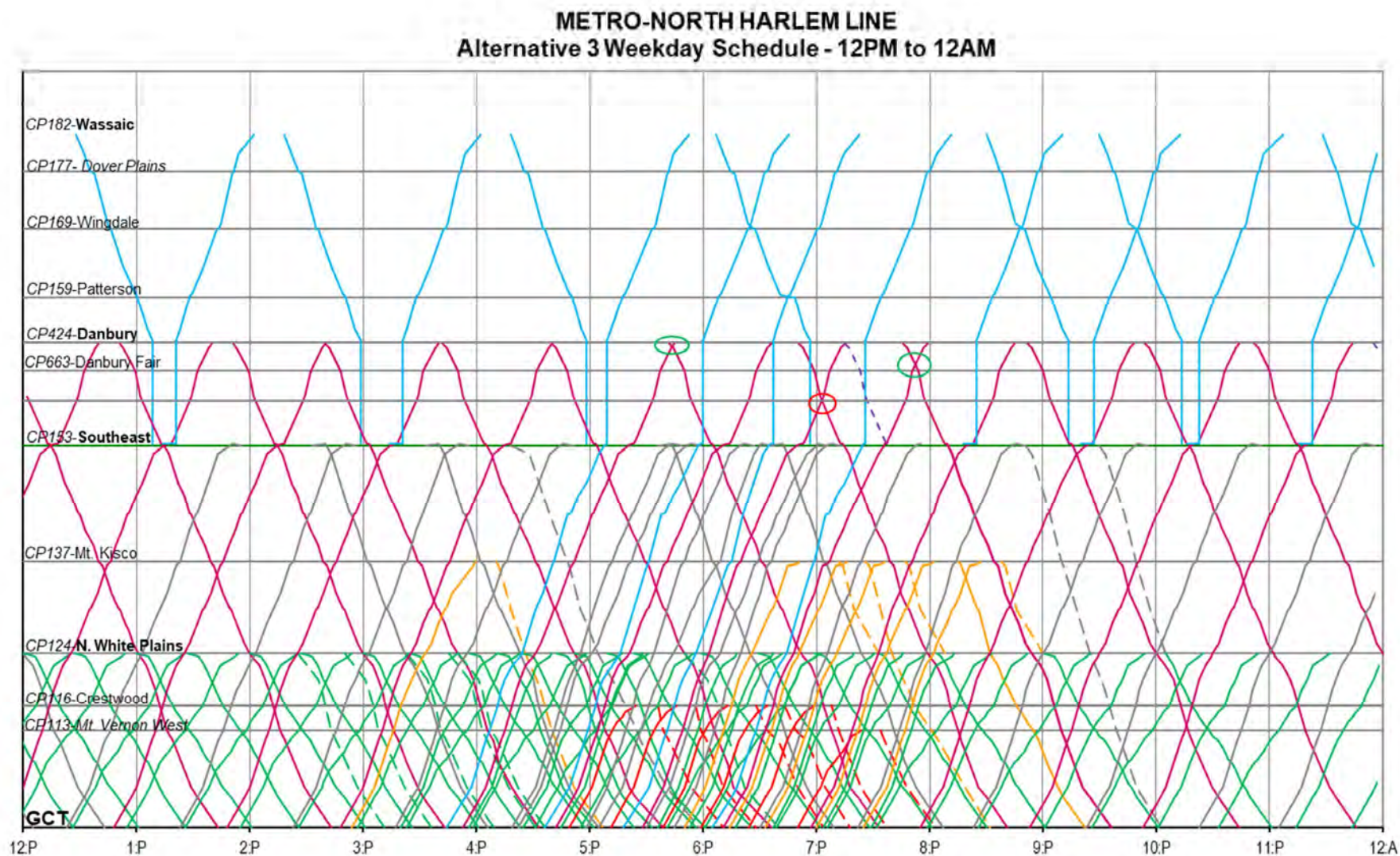
FIGURE 56. ALTERNATIVE 3 STRINGLINE DIAGRAM – 12PM TO 12 AM
