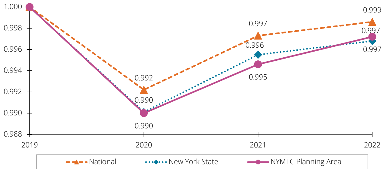
Figure 3.12 Comparative VMT Trends (in Log Values)
